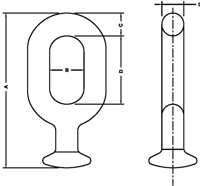
Ball & socket to IEC 16 MMB / 20 MM as specified
