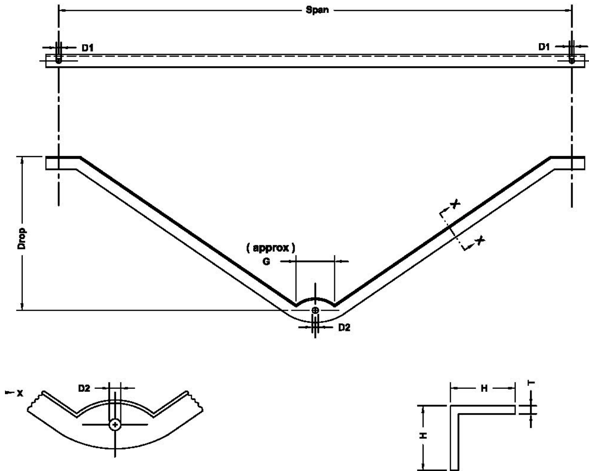
CENTRAL DETAIL
